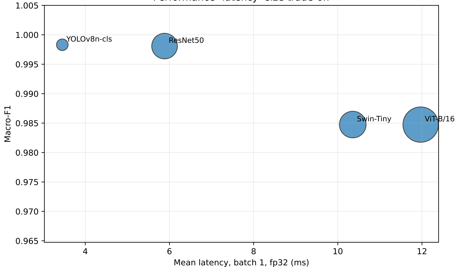
Performance--latency--size trade-off
