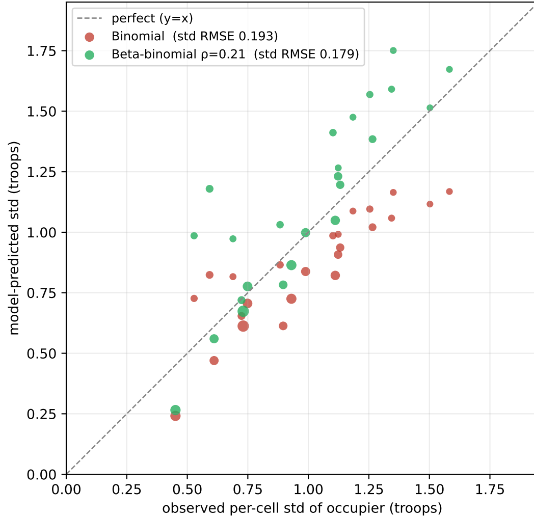
Capture-occupier overdispersion fix: beta-binomial ( p=0.21 ) vs plain binomial Mean UNCHANGED (win-rate unaffected) — only the spread is corrected to match the data Spread calibration, 24 capture cells ( n \geq 30, a \geq 4 ) Binomial sits BELOW y=x (too tight); beta-binomial lands on it
