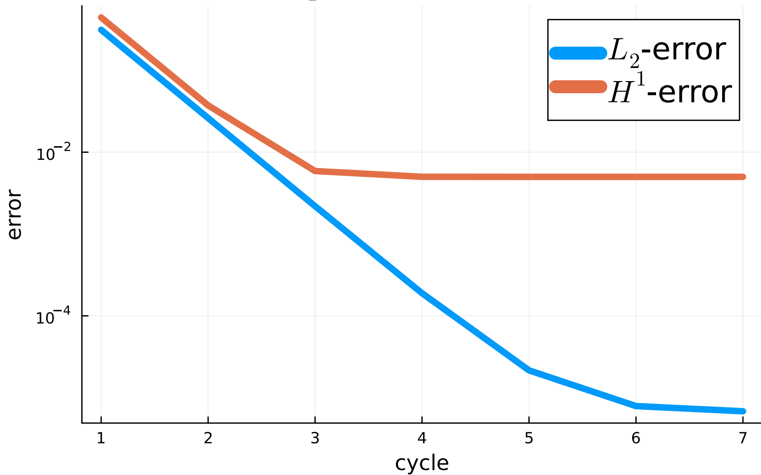
L_2/H^1 -norm of error
