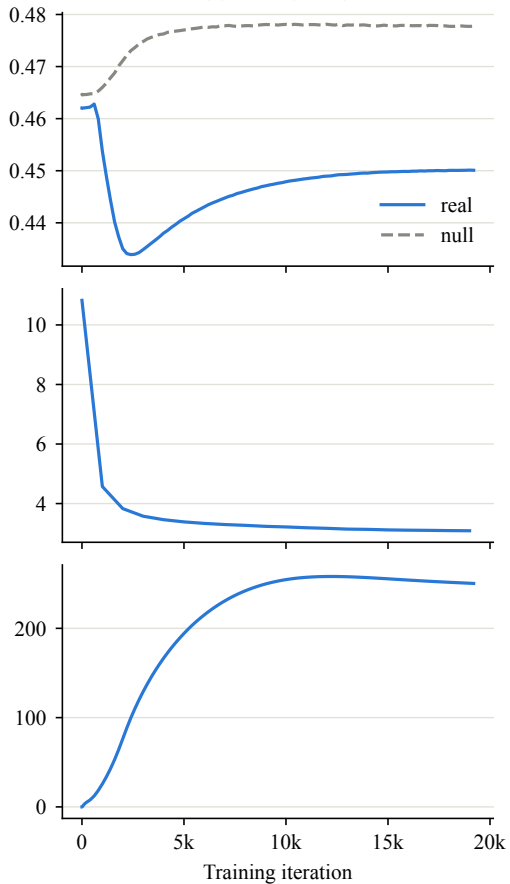
(b) Rich ( \alpha = 1 )
