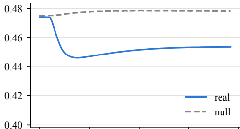
(b) Rich (init scale = 1)
