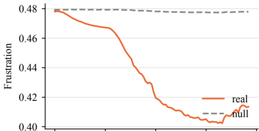
(a) Lazy (init scale = 5)
