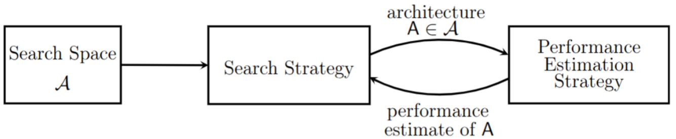
Figure 2.1: Overview of the three components of NAS from [11].
