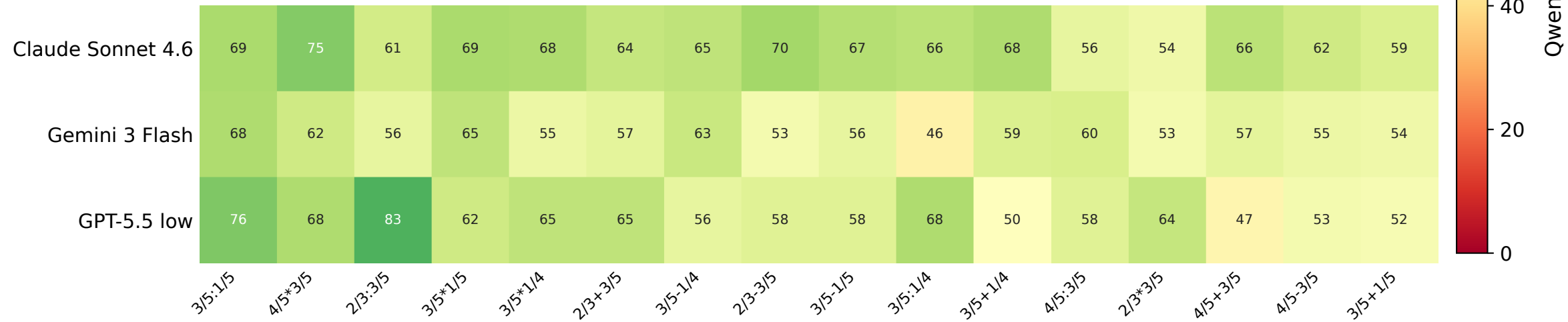
Fraction: Qwen preference by problem
