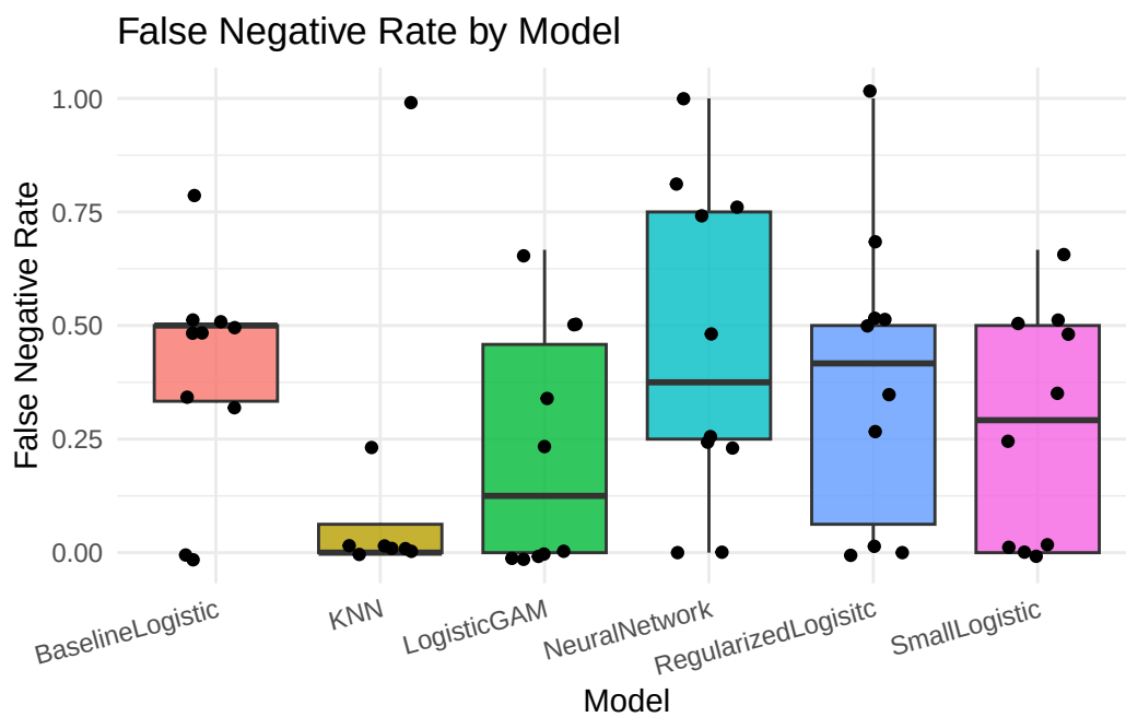
Figure 3: False Negative Rate by Model for Each Fold
