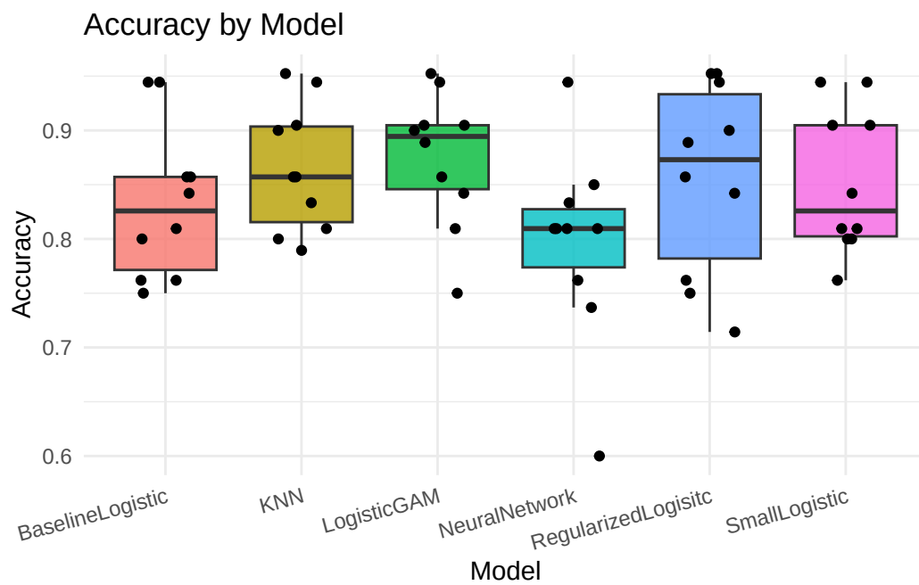
Figure 1: Accuracy by Model for Each Fold
