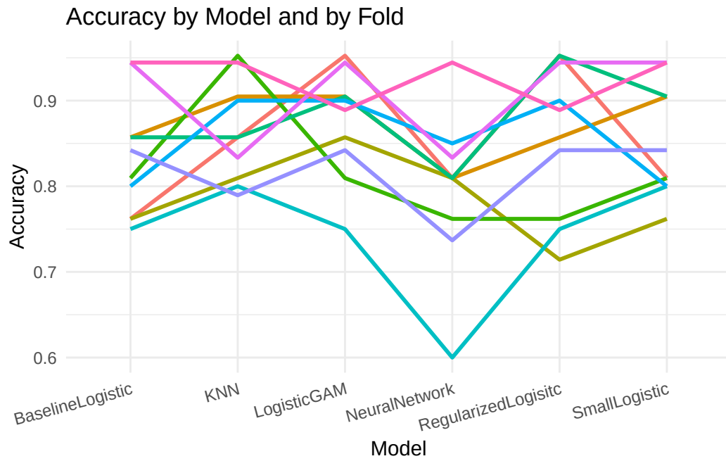
Figure 4: Accuracy by Model and by Fold
