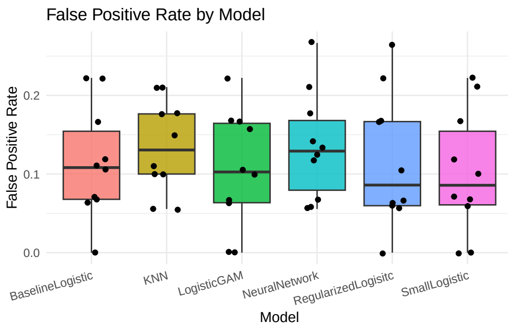
Figure 2: False Positive Rate by Model for Each Fold
