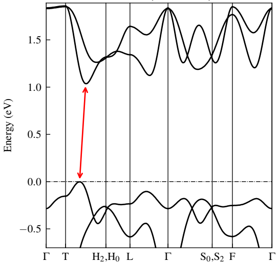
LiCoO 2 (ISCD 51767)
