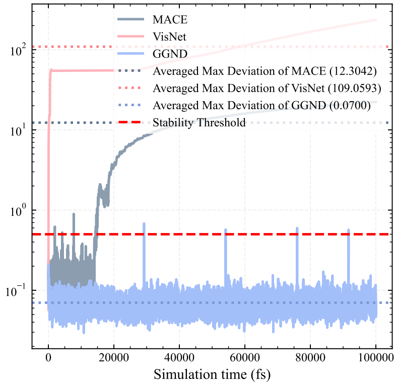
Stability on 1200 K MD
