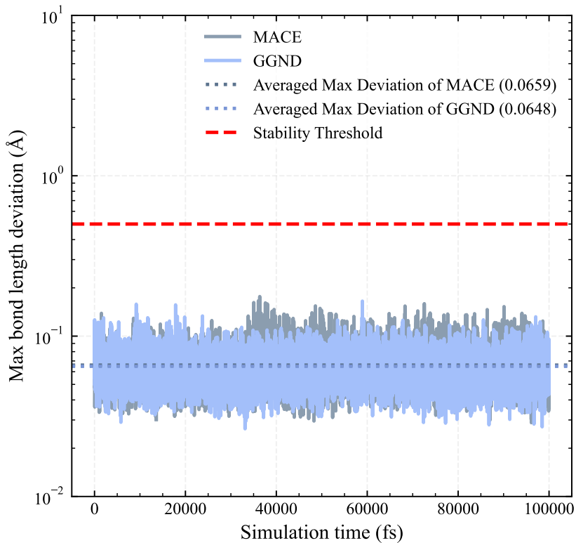
Stability on 600 K MD
