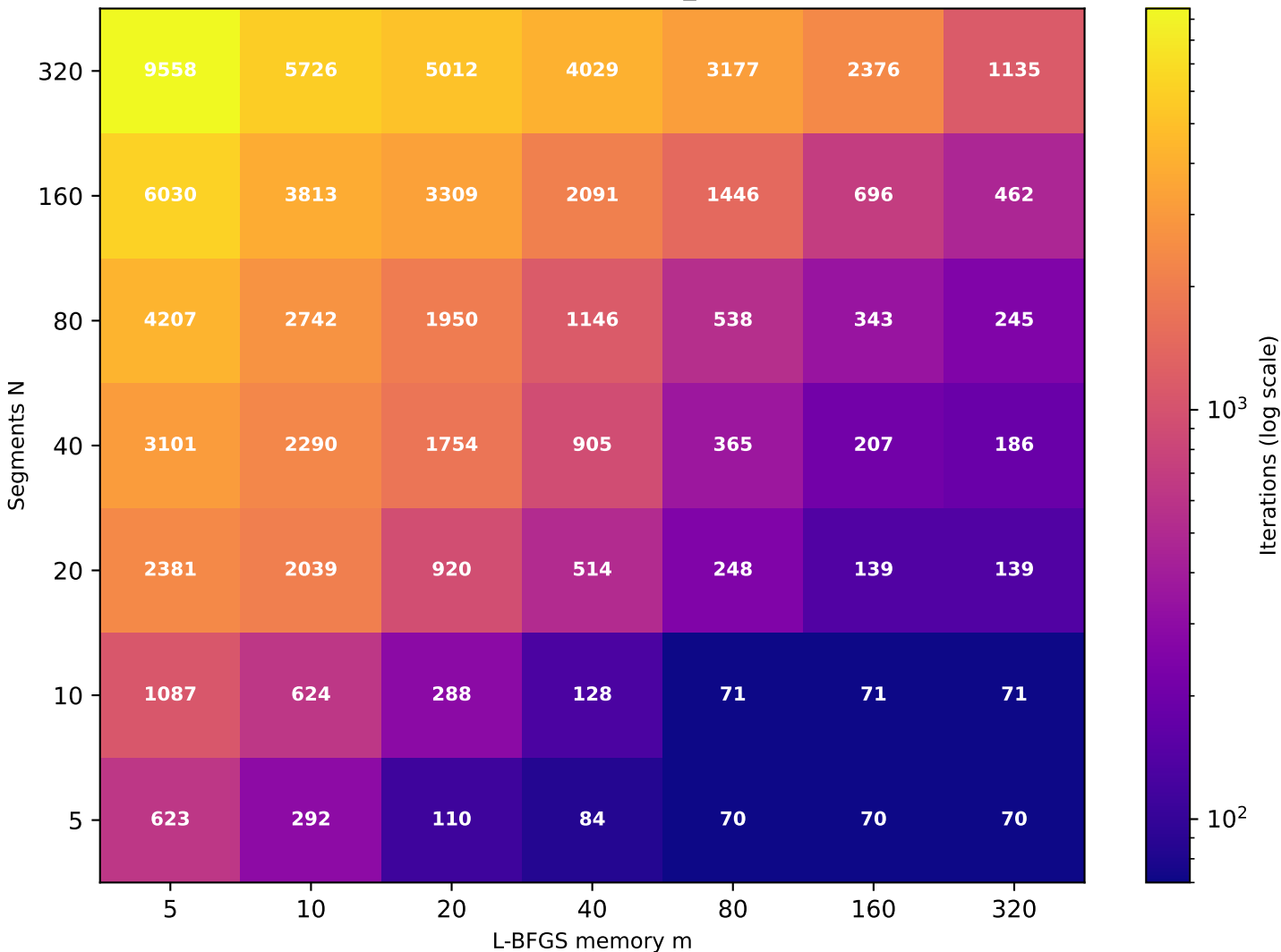
Recurrence T \approx 9.07 (target T=10 , rec_id=4) [49/49 converged]
