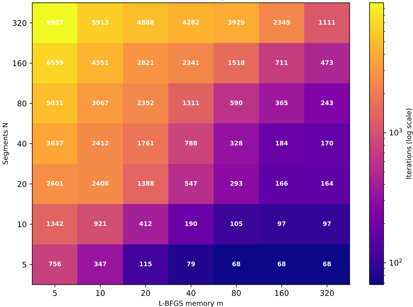
Recurrence T \approx 9.07 (target T=10 , rec_id=6) [49/49 converged]
