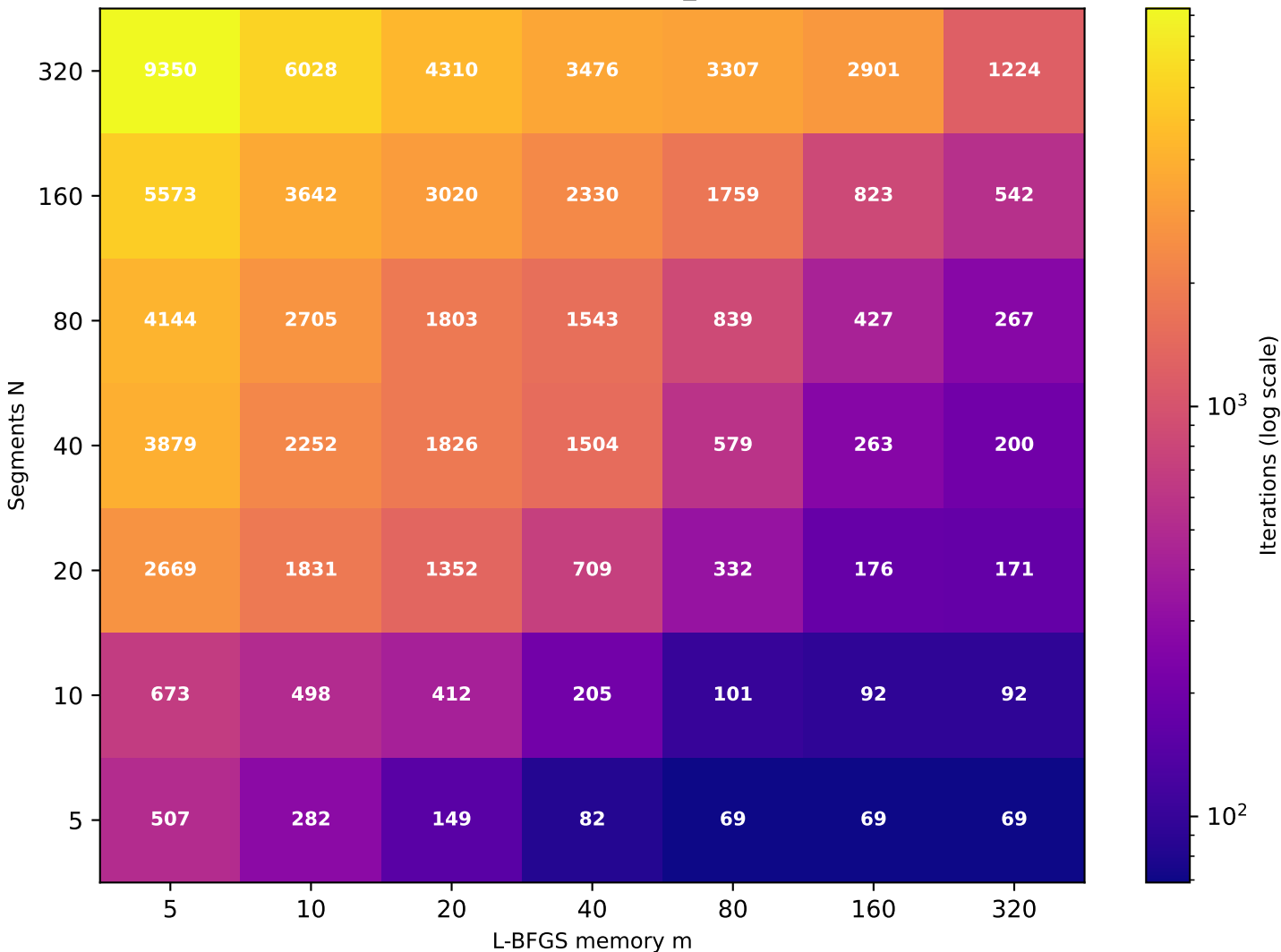
Recurrence T \approx 11.46 (target T=10 , rec_id=16) [49/49 converged]
