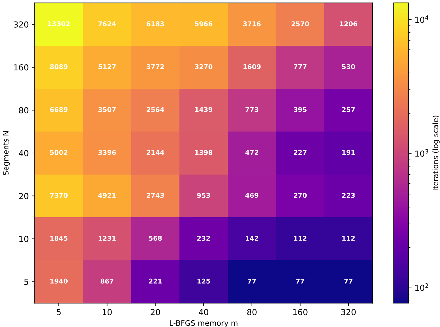
Recurrence T \approx 10.55 (target T=10 , rec_id=17) [49/49 converged]
