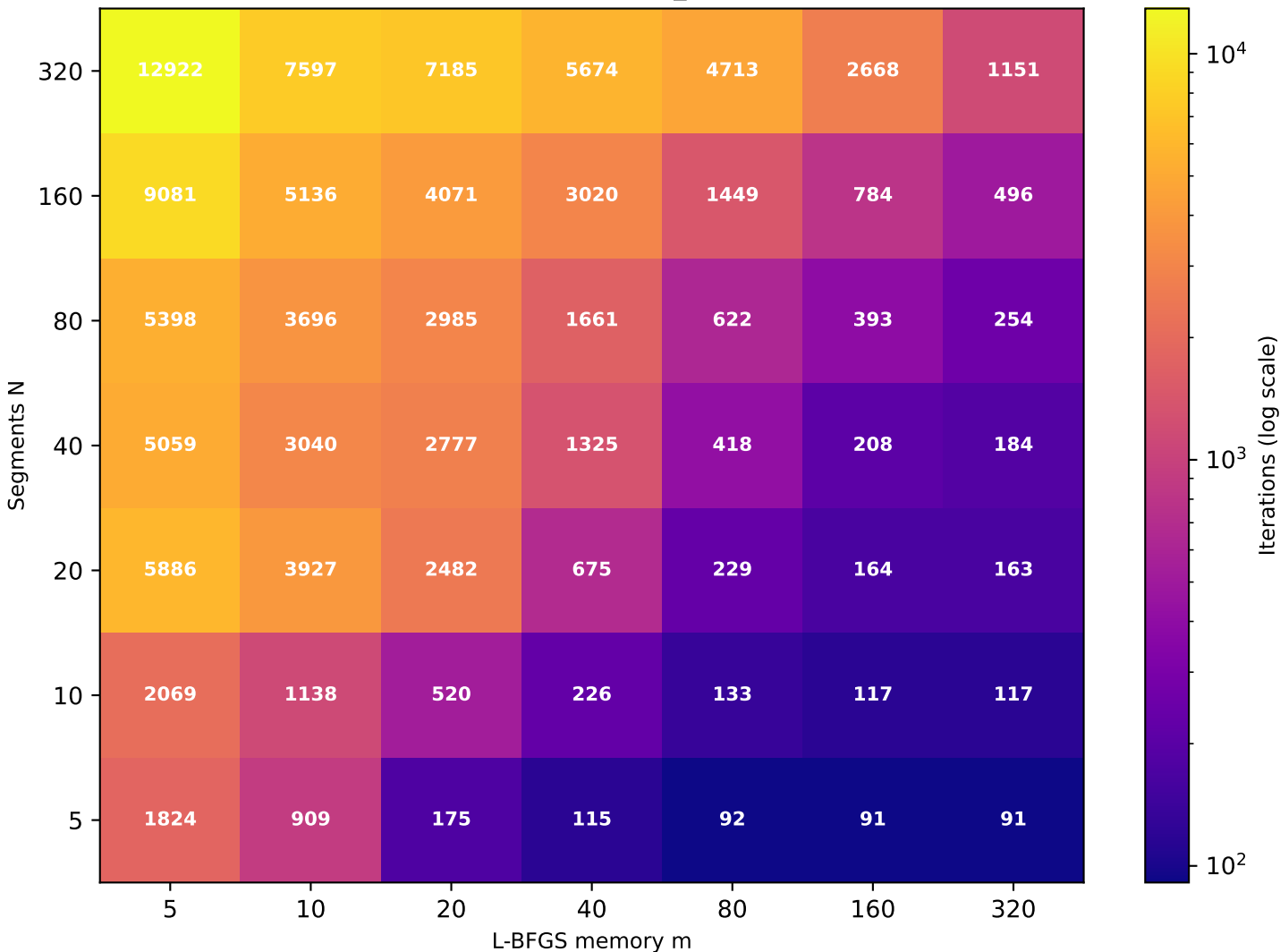
Recurrence T \approx 9.71 (target T=10 , rec_id=20) [49/49 converged]
