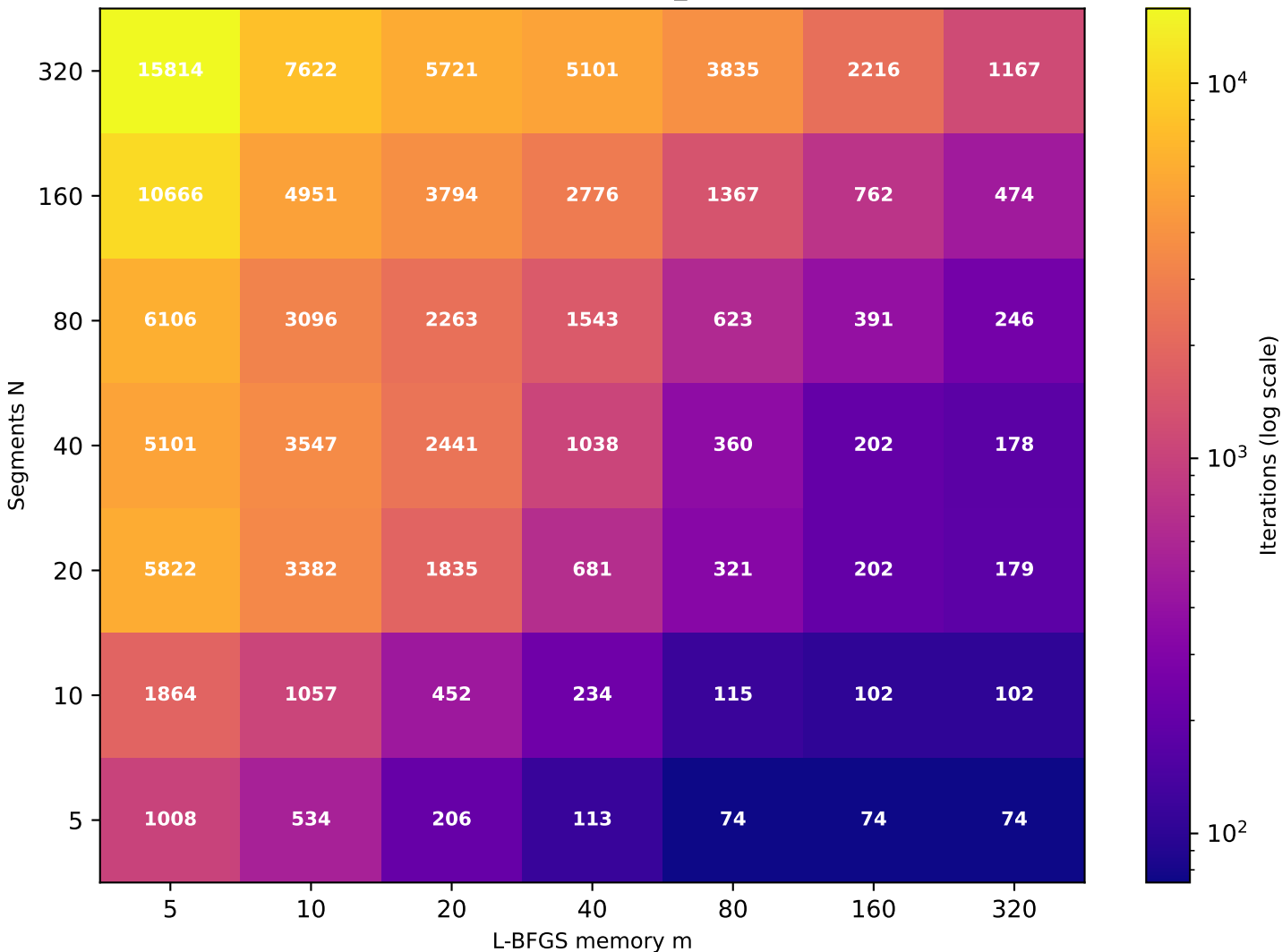
Recurrence T \approx 9.62 (target T=10 , rec_id=21) [49/49 converged]
