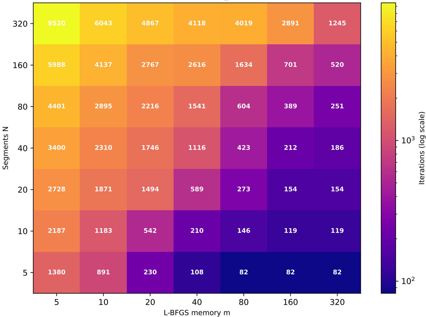
Recurrence T \approx 9.20 (target T=10 , rec_id=24) [49/49 converged]
