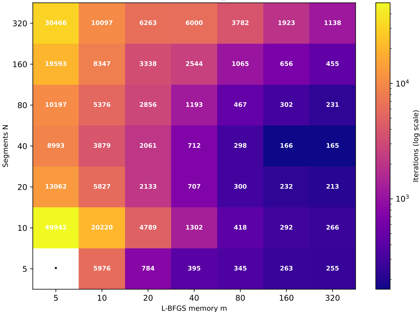
Recurrence T \approx 8.64 (target T=10 , rec_id=27) [48/49 converged]
