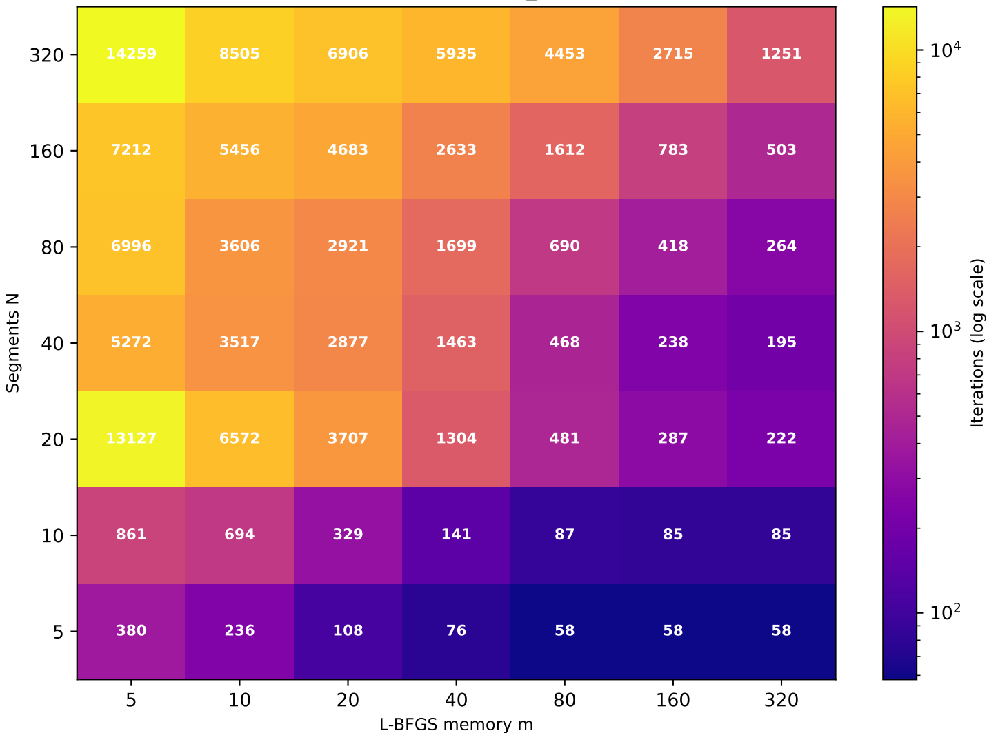
Recurrence T \approx 10.55 (target T=10 , rec_id=29) [49/49 converged]
