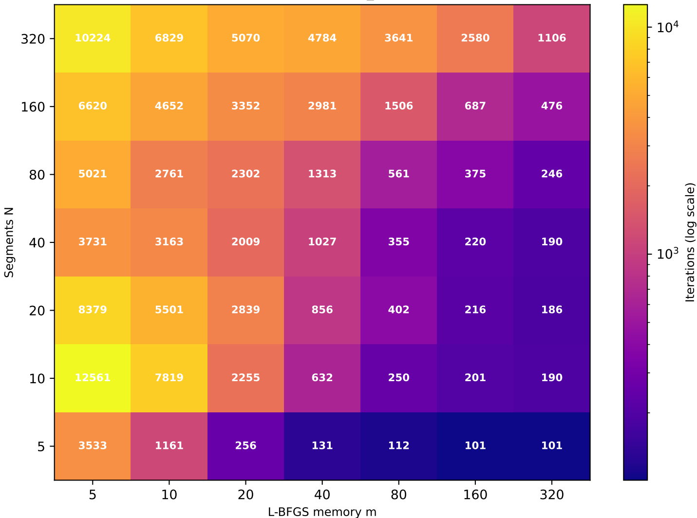
Recurrence T \approx 9.07 (target T=10 , rec_id=31) [49/49 converged]
