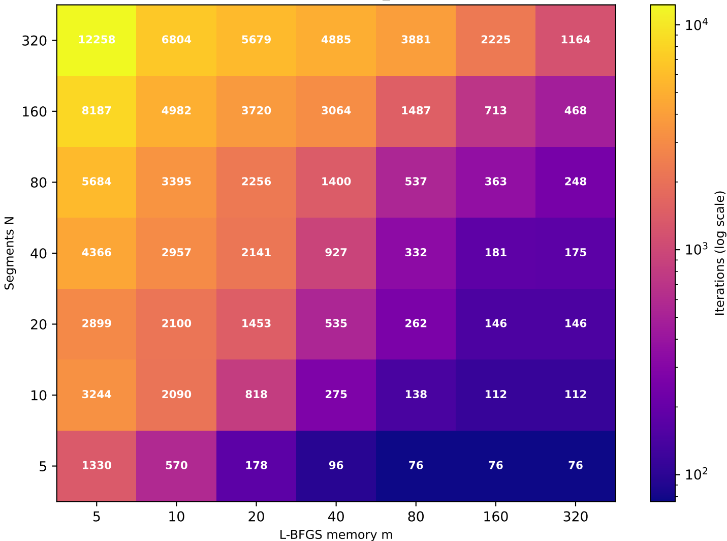
Recurrence T \approx 8.32 (target T=10 , rec_id=34) [49/49 converged]
