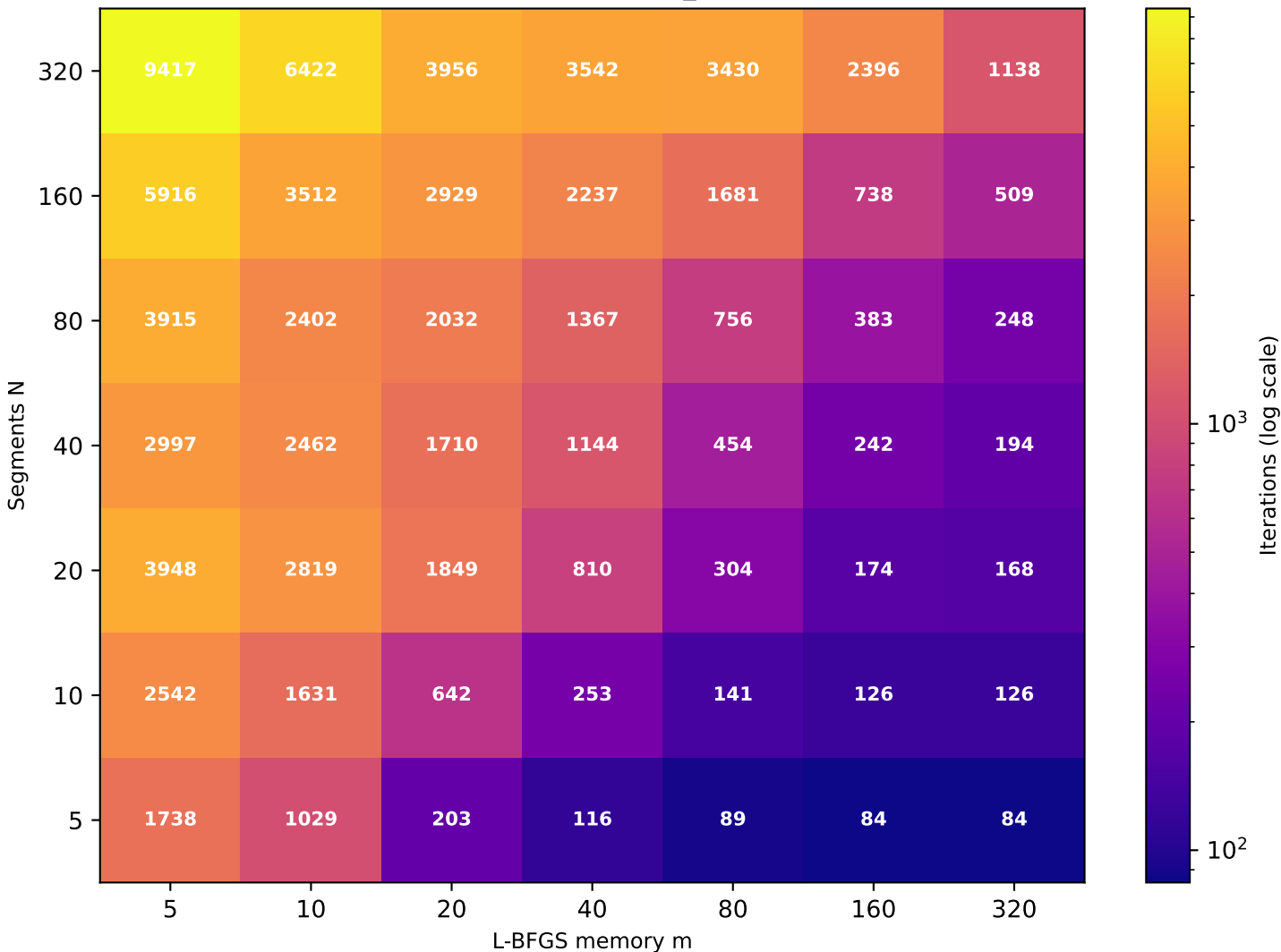
Recurrence T \approx 10.01 (target T=10 , rec_id=37) [49/49 converged]
