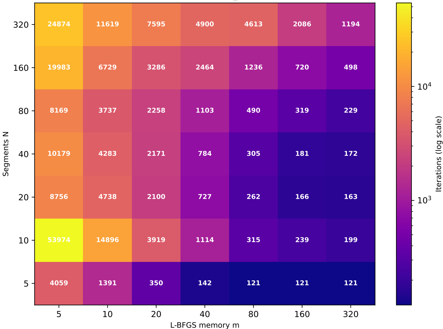
Recurrence T \approx 8.64 (target T=10 , rec_id=48) [49/49 converged]
