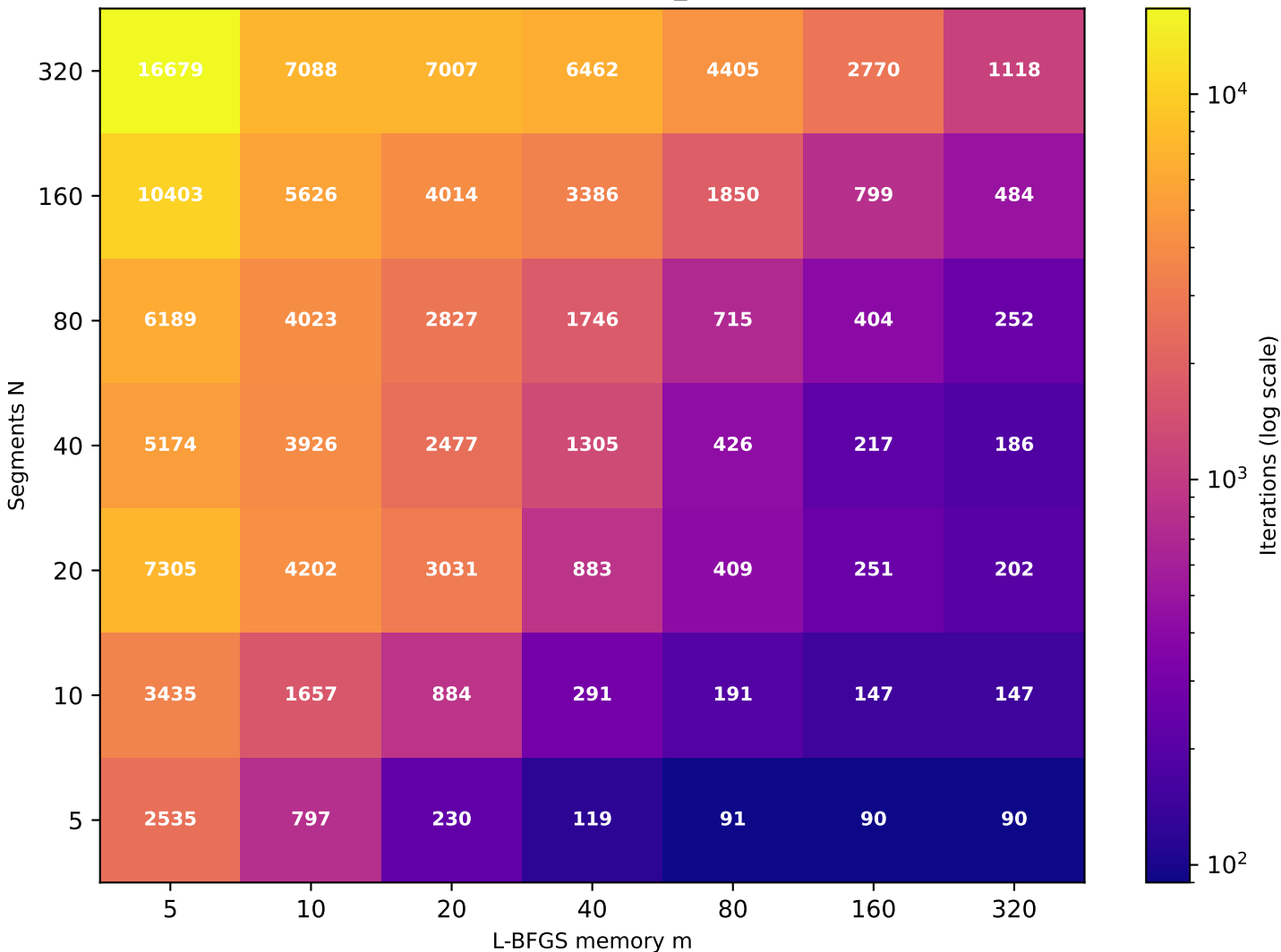
Recurrence T \approx 9.76 (target T=10 , rec_id=51) [49/49 converged]
