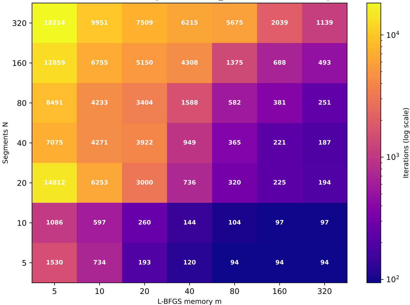
Recurrence T \approx 10.19 (target T=10 , rec_id=57) [49/49 converged]
