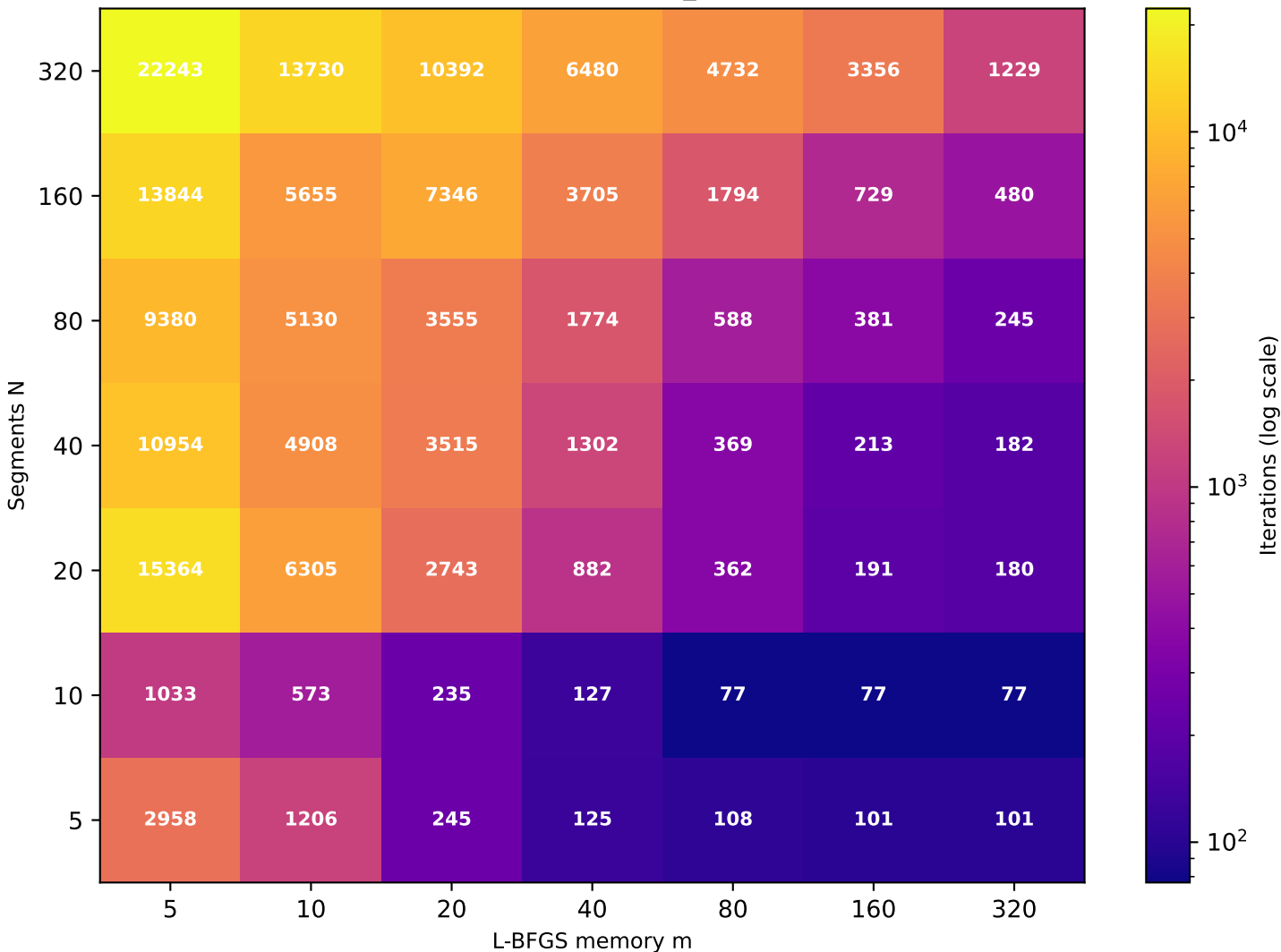
Recurrence T \approx 10.16 (target T=10 , rec_id=60) [49/49 converged]
