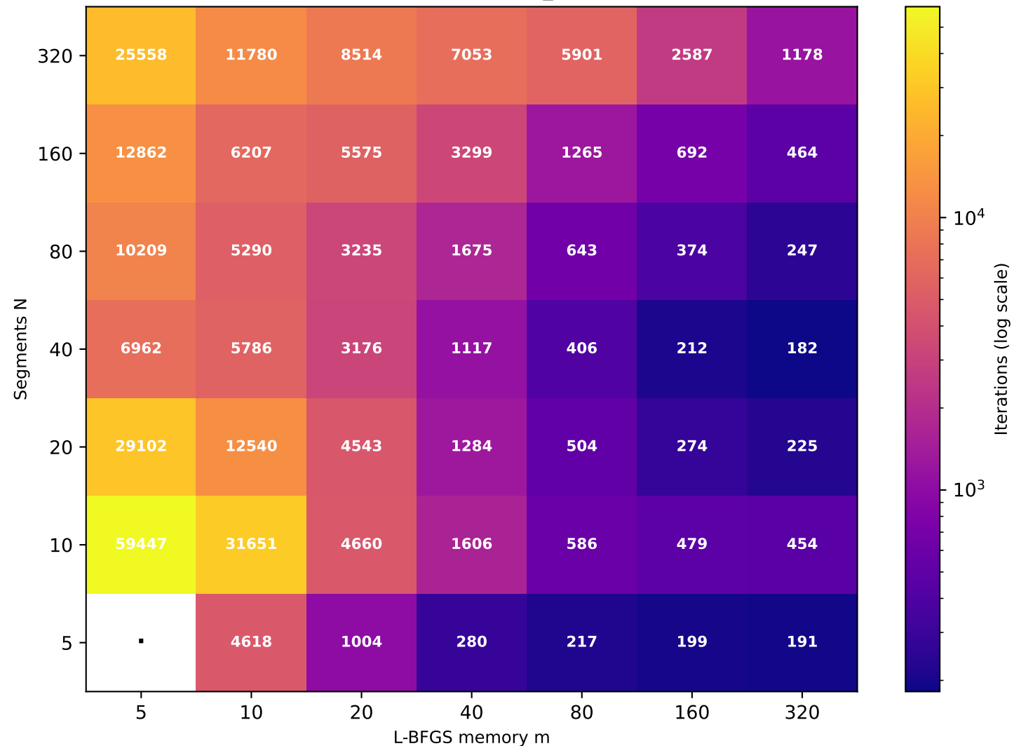
Recurrence T \approx 10.16 (target T=10 , rec_id=61) [48/49 converged]
