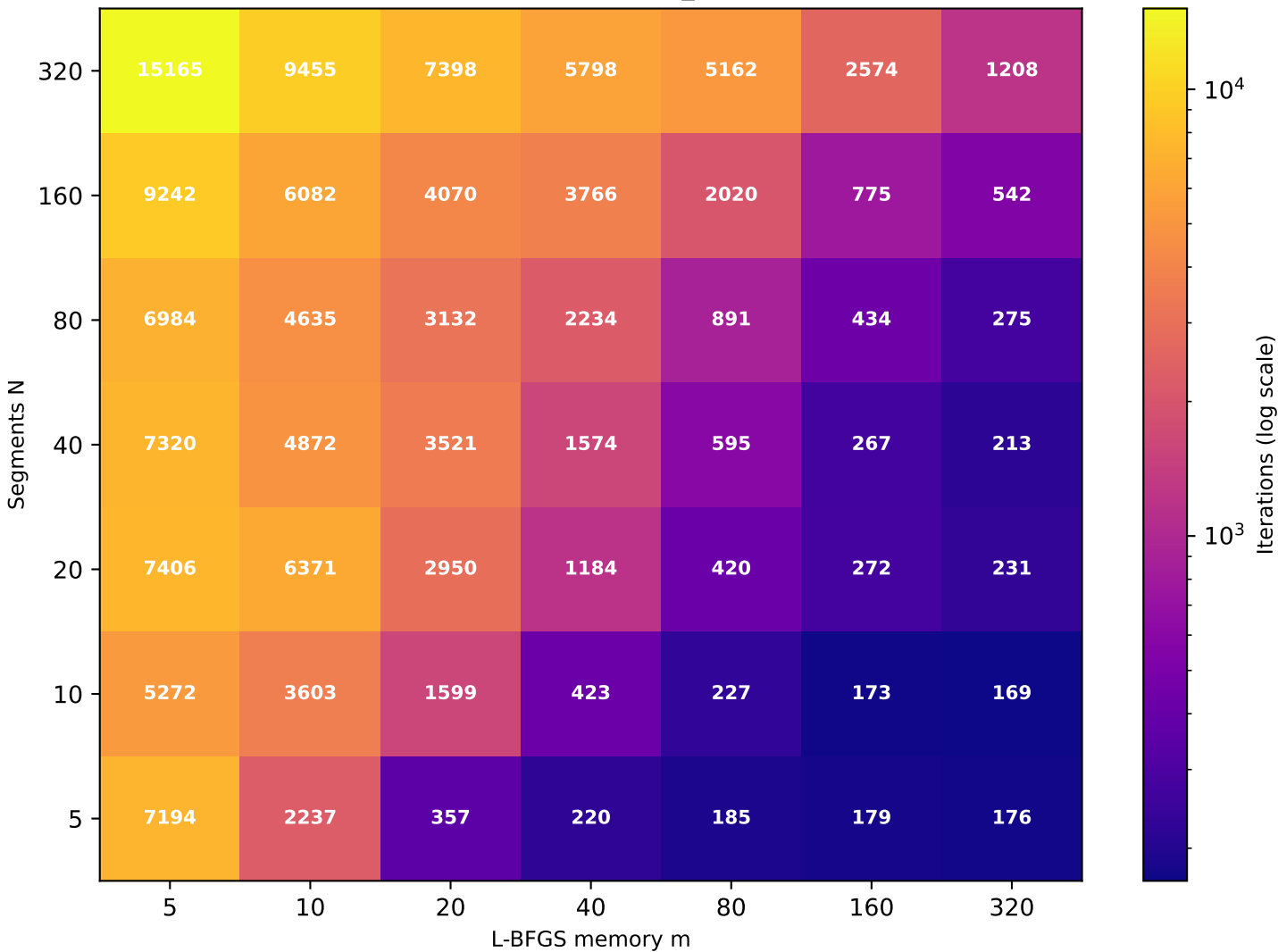
Recurrence T \approx 11.99 (target T=10 , rec_id=62) [49/49 converged]
