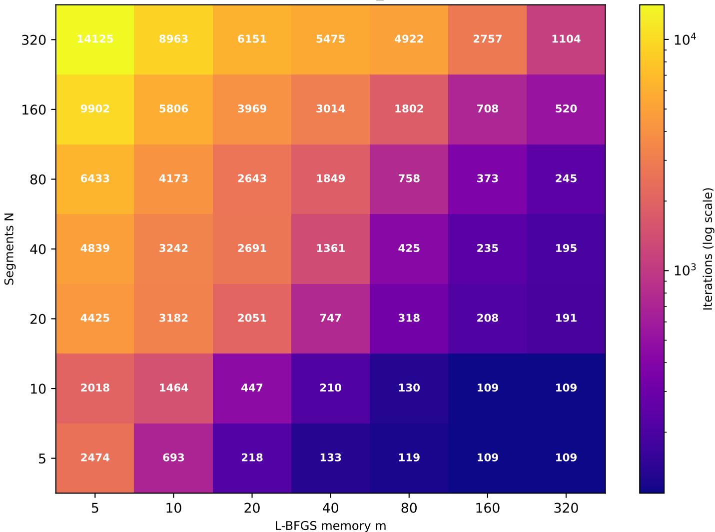
Recurrence T \approx 9.86 (target T=10 , rec_id=64) [49/49 converged]
