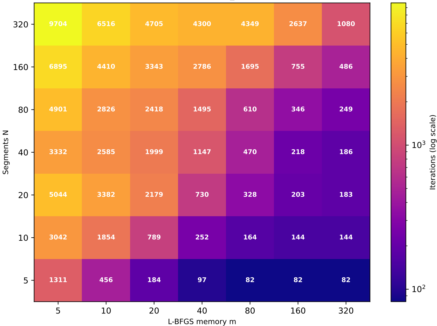
Recurrence T \approx 9.15 (target T=10 , rec_id=65) [49/49 converged]
