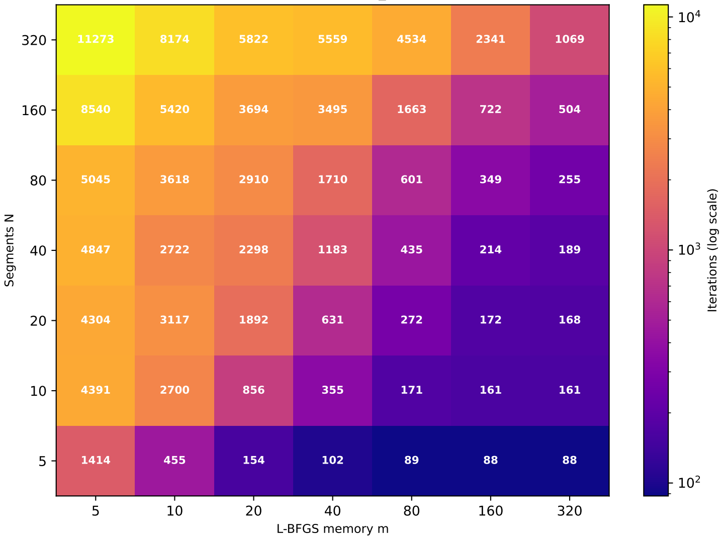
Recurrence T \approx 9.11 (target T=10 , rec_id=66) [49/49 converged]
