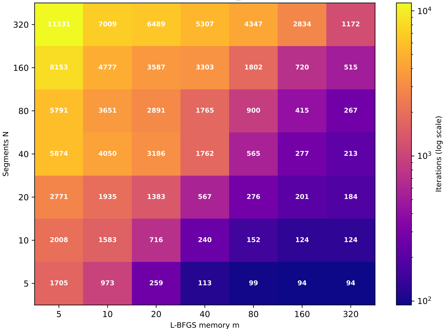
Recurrence T \approx 11.39 (target T=10 , rec_id=67) [49/49 converged]
