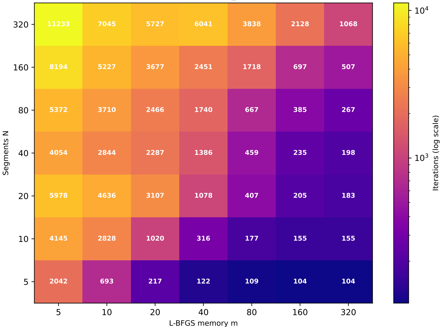
Recurrence T \approx 9.93 (target T=10 , rec_id=74) [49/49 converged]
