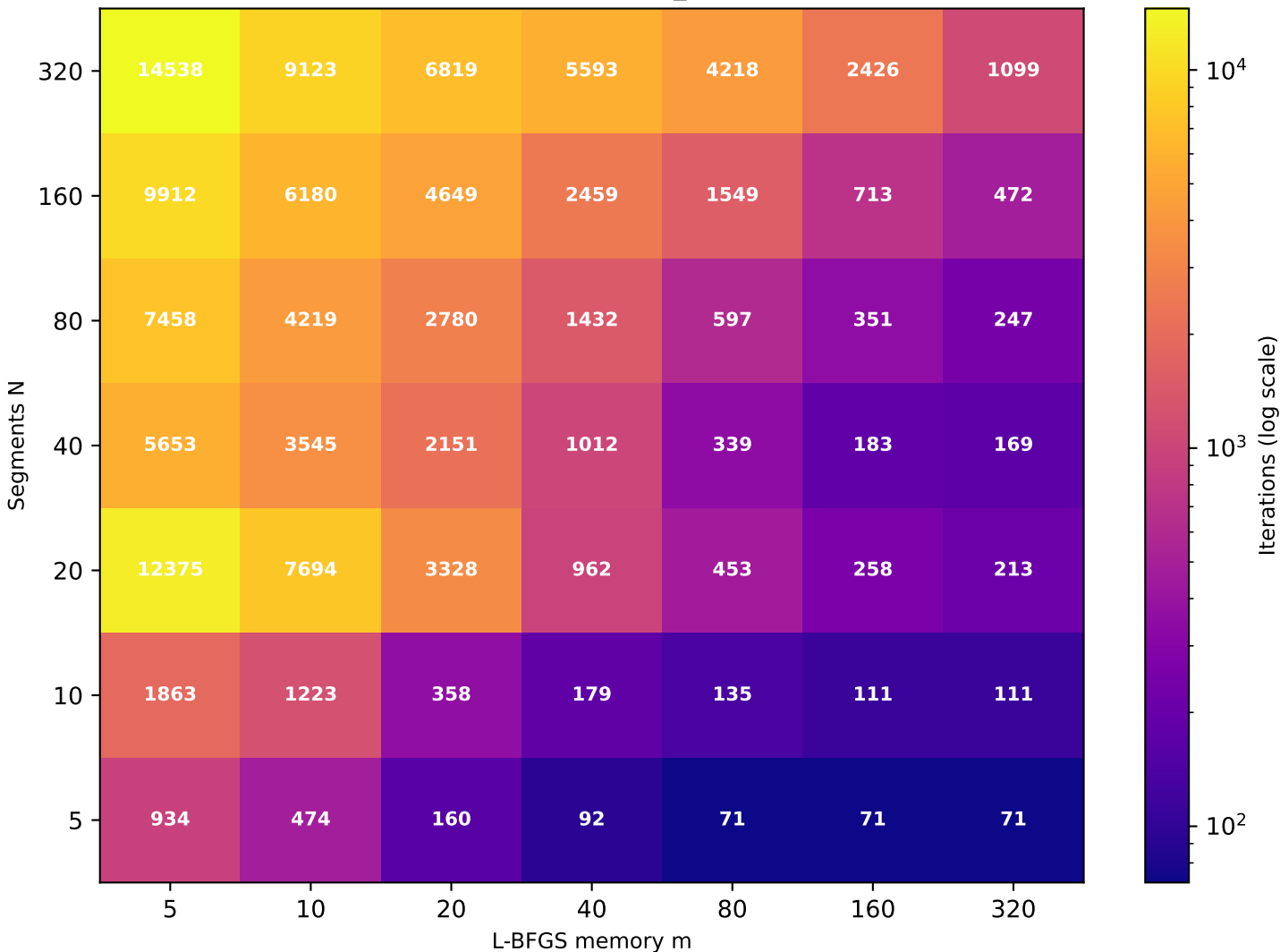
Recurrence T \approx 8.99 (target T=10 , rec_id=75) [49/49 converged]
