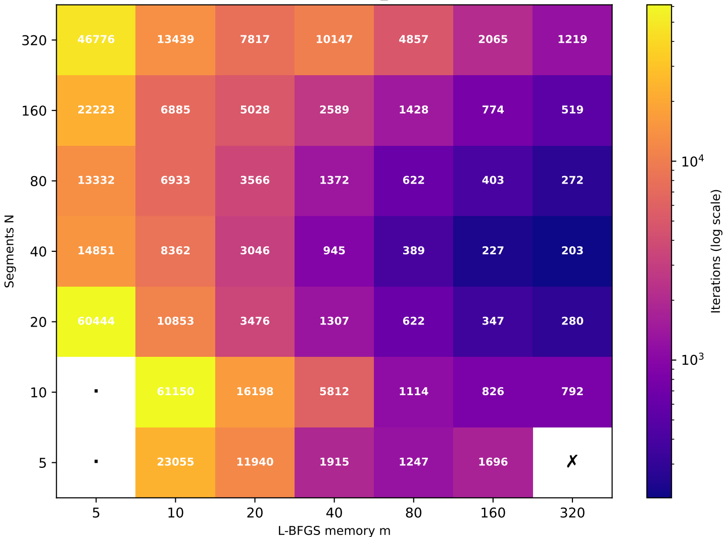
Recurrence T \approx 9.98 (target T=10 , rec_id=78) [46/49 converged]
