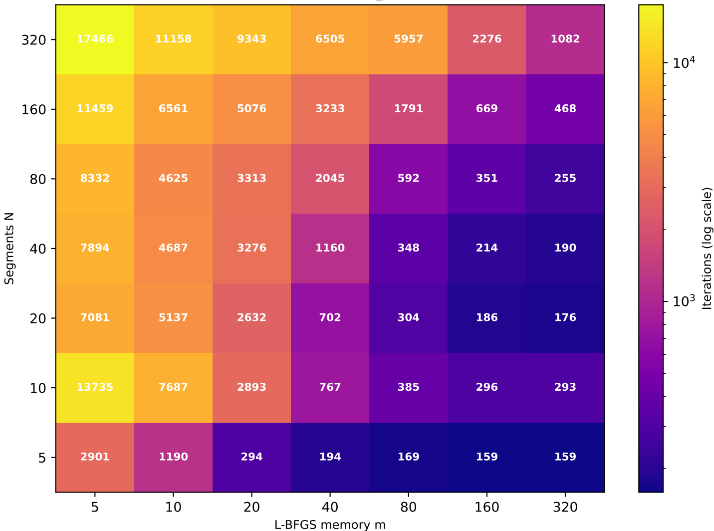
Recurrence T \approx 9.62 (target T=10 , rec_id=79) [49/49 converged]
