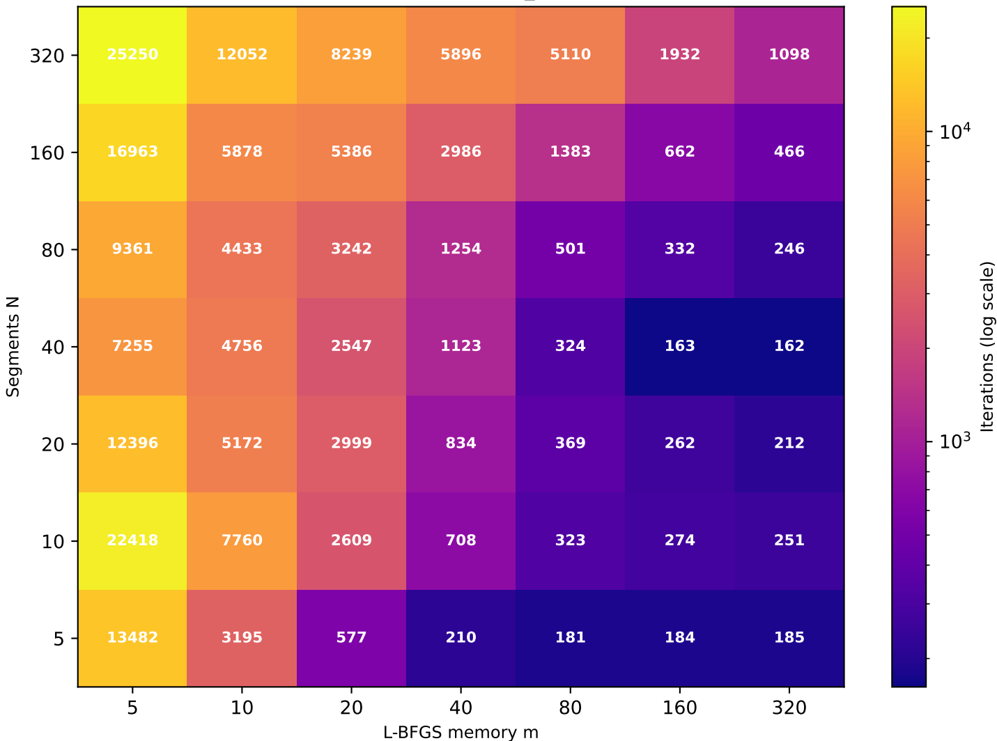
Recurrence T \approx 8.84 (target T=10 , rec_id=82) [49/49 converged]
