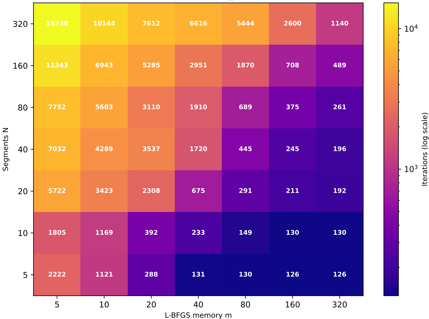
Recurrence T \approx 10.42 (target T=10 , rec_id=84) [49/49 converged]
