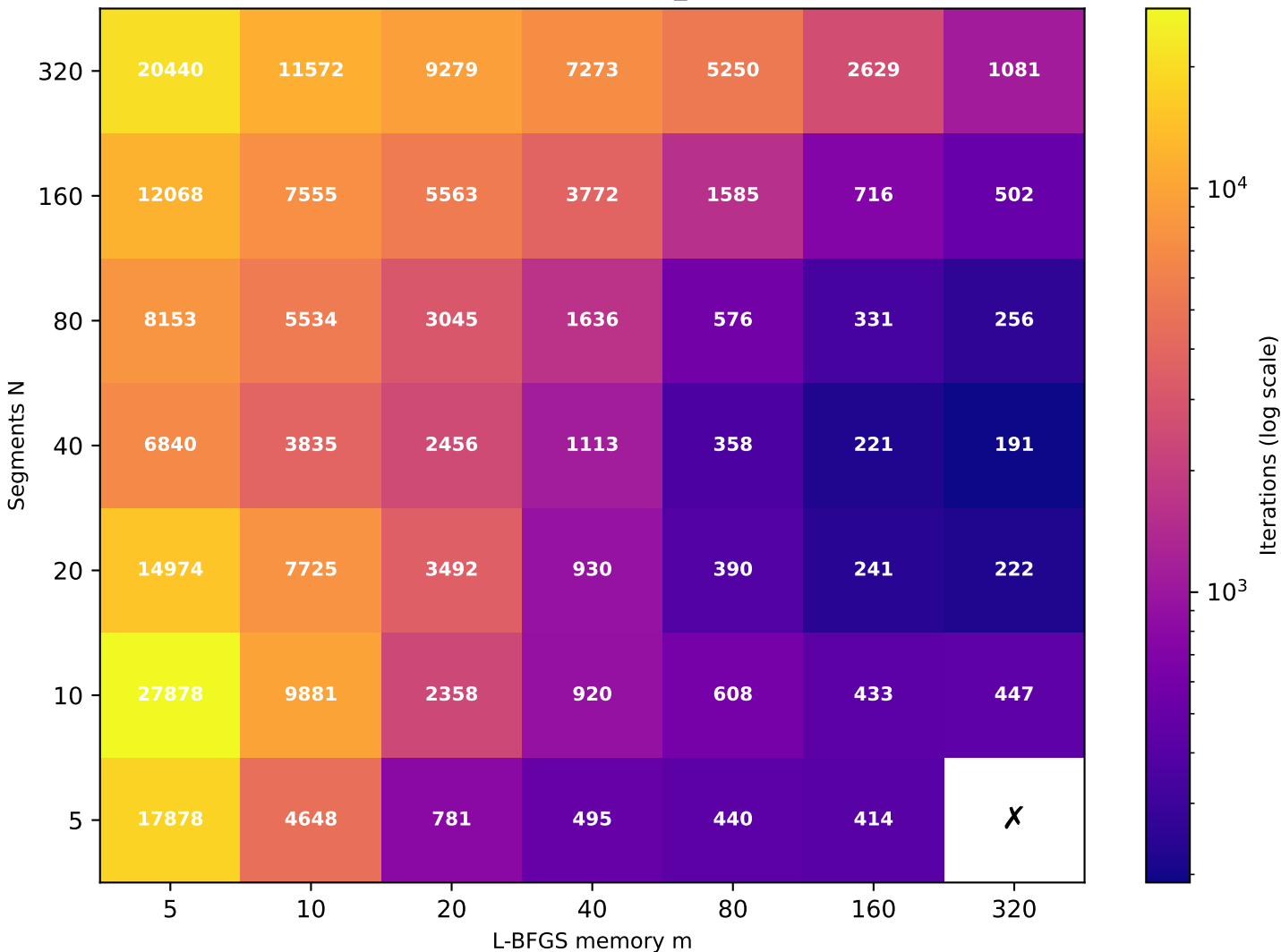
Recurrence T \approx 8.94 (target T=10 , rec_id=86) [48/49 converged]
