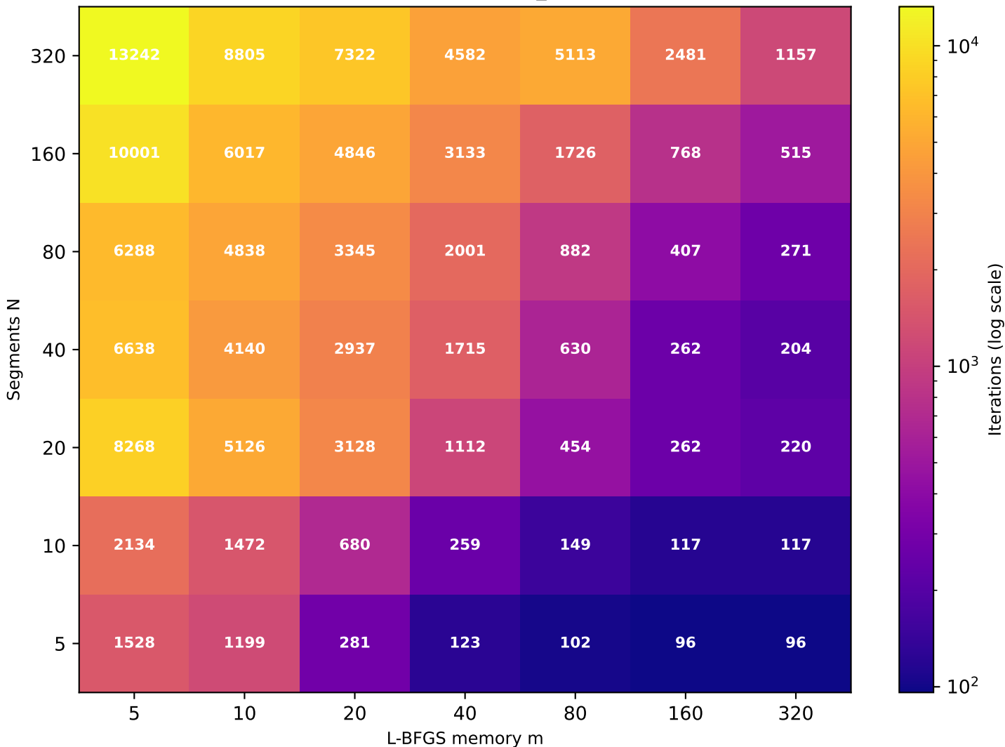
Recurrence T \approx 11.31 (target T=10 , rec_id=90) [49/49 converged]
