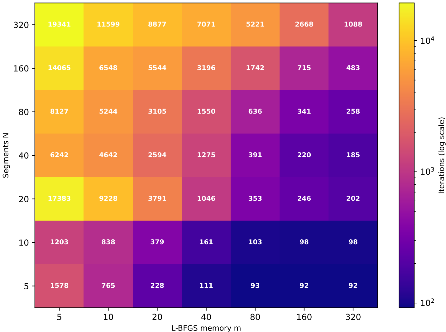
Recurrence T \approx 9.72 (target T=10 , rec_id=94) [49/49 converged]
