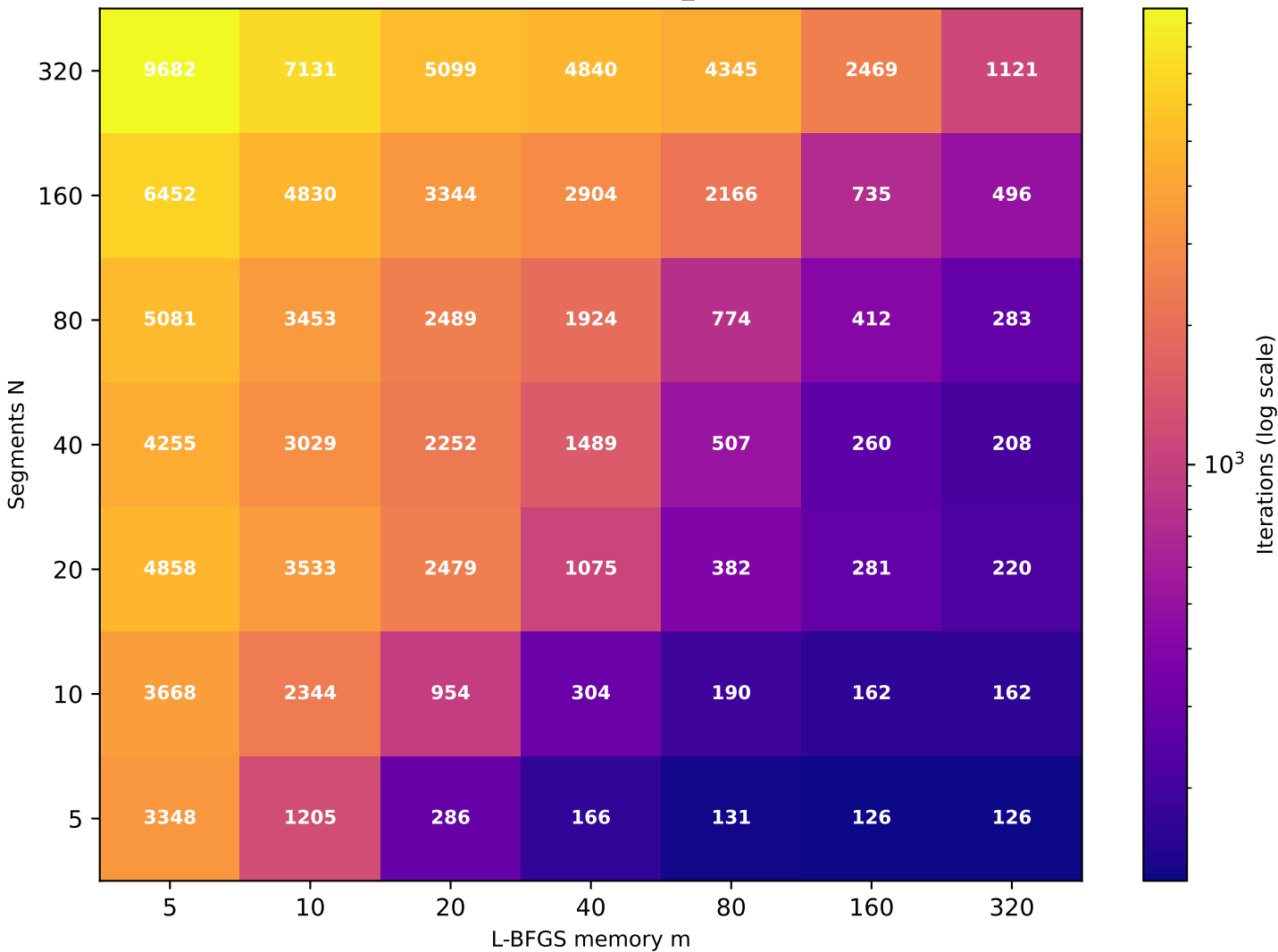
Recurrence T \approx 10.71 (target T=10 , rec_id=97) [49/49 converged]
