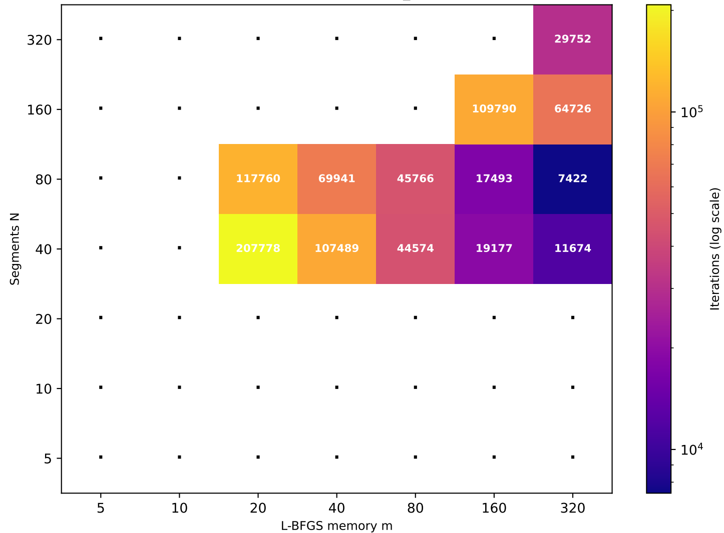
Recurrence T \approx 161.75 (target T=160 , rec_id=5) [13/49 converged]
