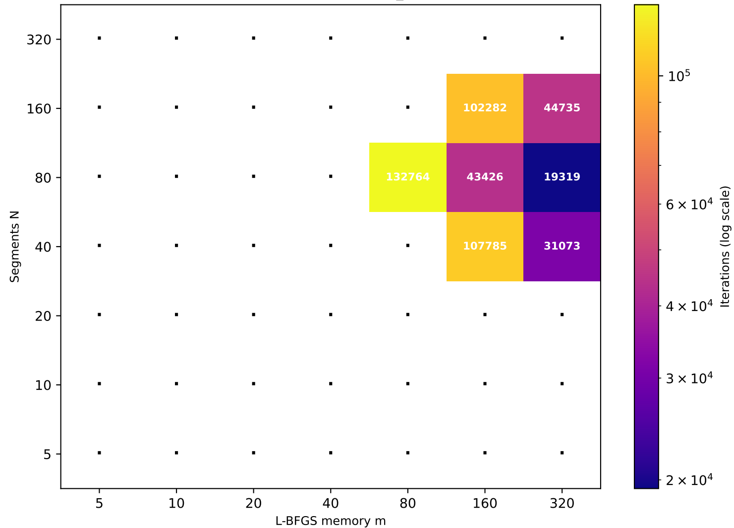
Recurrence T \approx 161.76 (target T=160 , rec_id=11) [7/49 converged]
