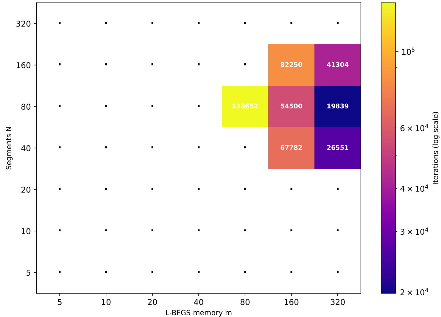
Recurrence T \approx 162.31 (target T=160 , rec_id=17) [7/49 converged]
