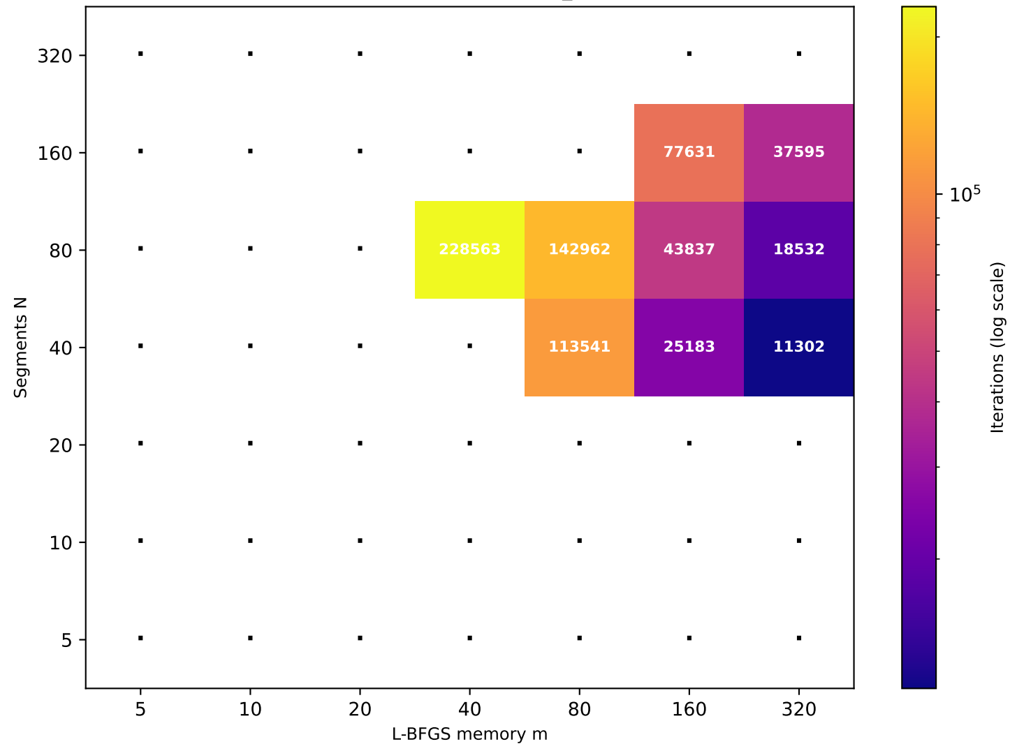
Recurrence T \approx 159.92 (target T=160 , rec_id=21) [9/49 converged]
