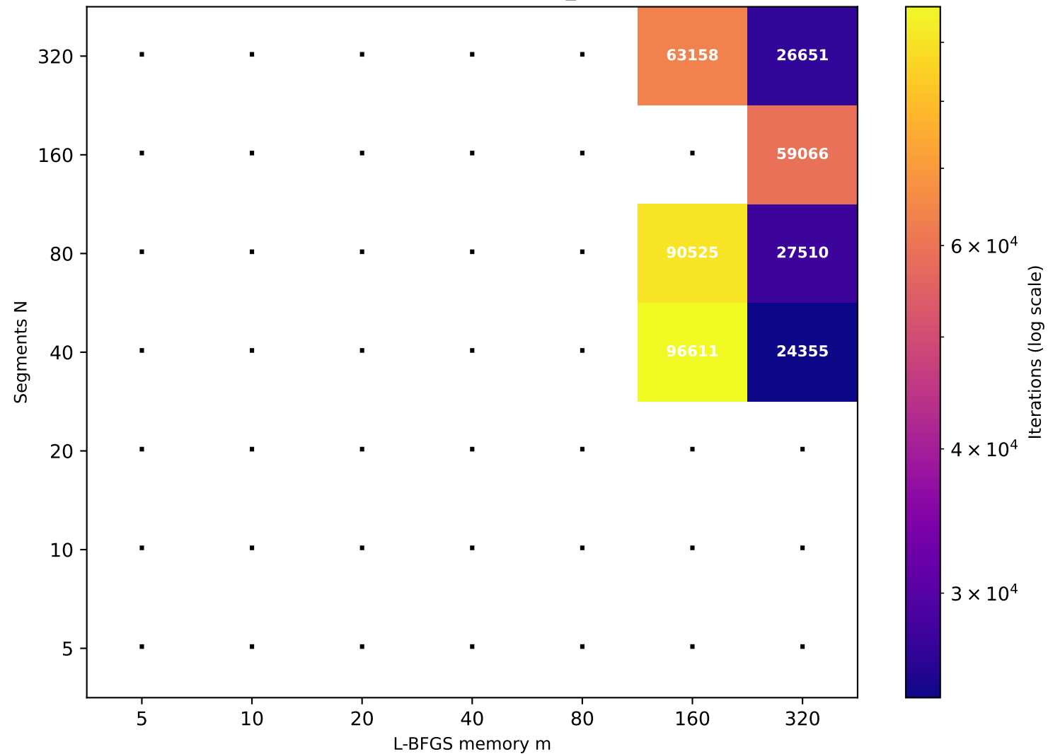
Recurrence T \approx 161.86 (target T=160 , rec_id=31) [7/49 converged]
