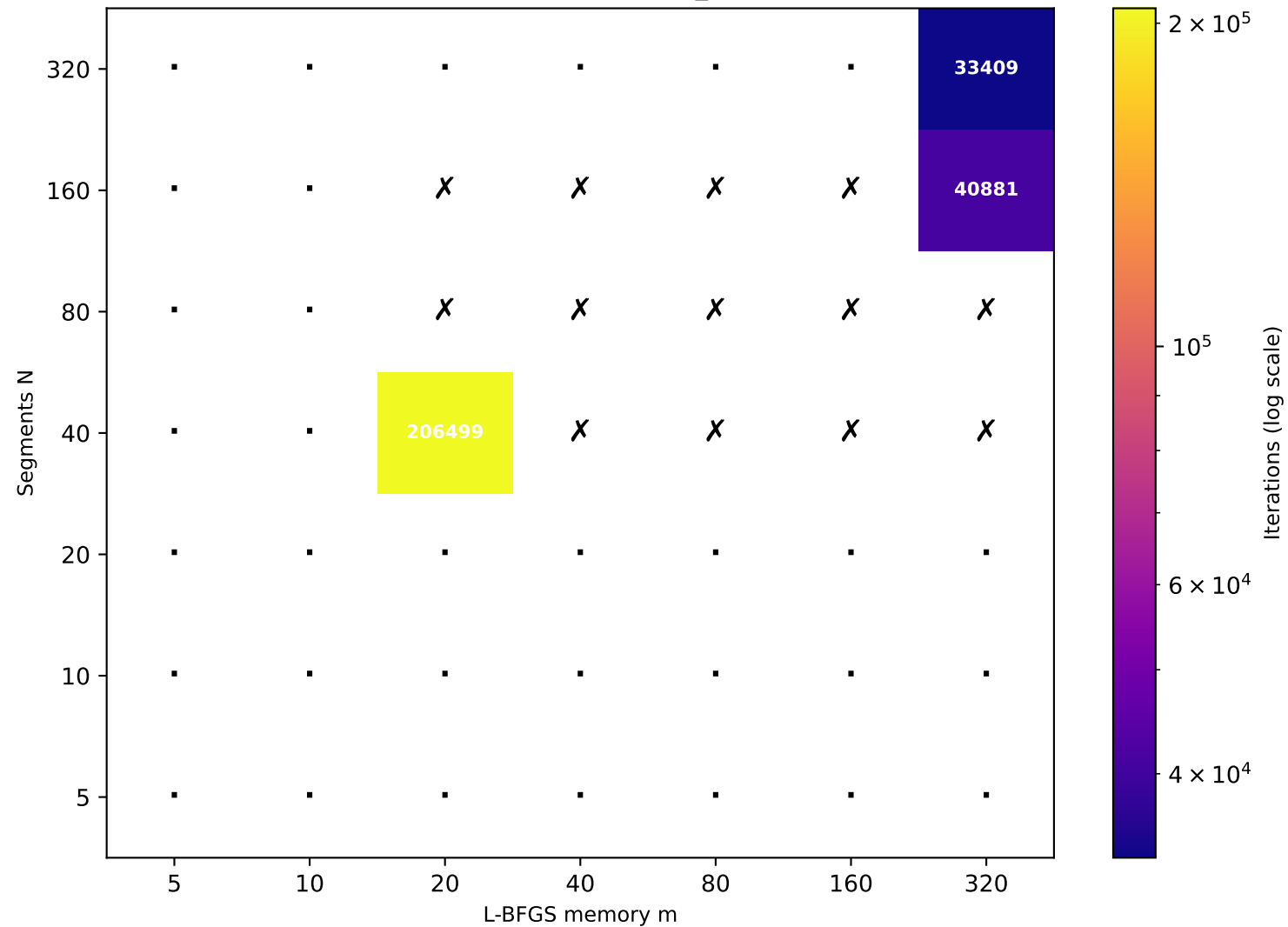
Recurrence T \approx 158.55 (target T=160 , rec_id=36) [3/49 converged]
