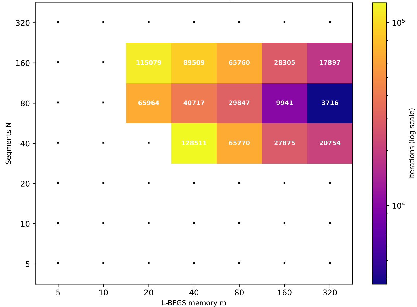
Recurrence T \approx 160.12 (target T=160 , rec_id=41) [14/49 converged]
