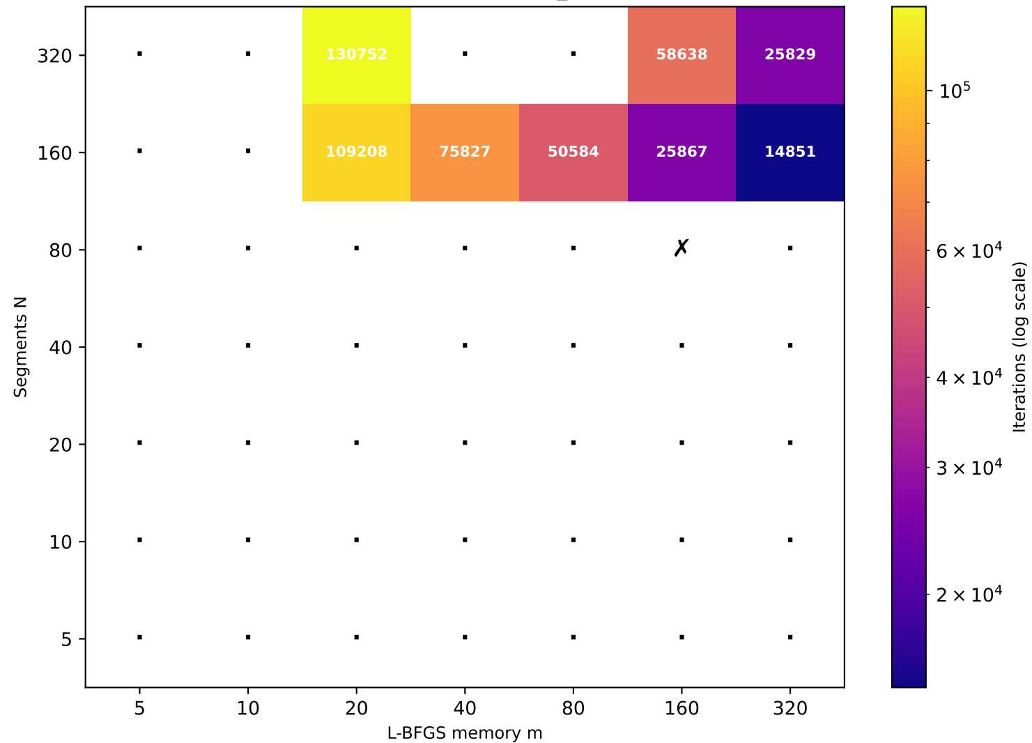
Recurrence T \approx 159.43 (target T=160 , rec_id=59) [8/49 converged]
